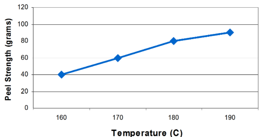
Typical Peel Strength (Mean)
